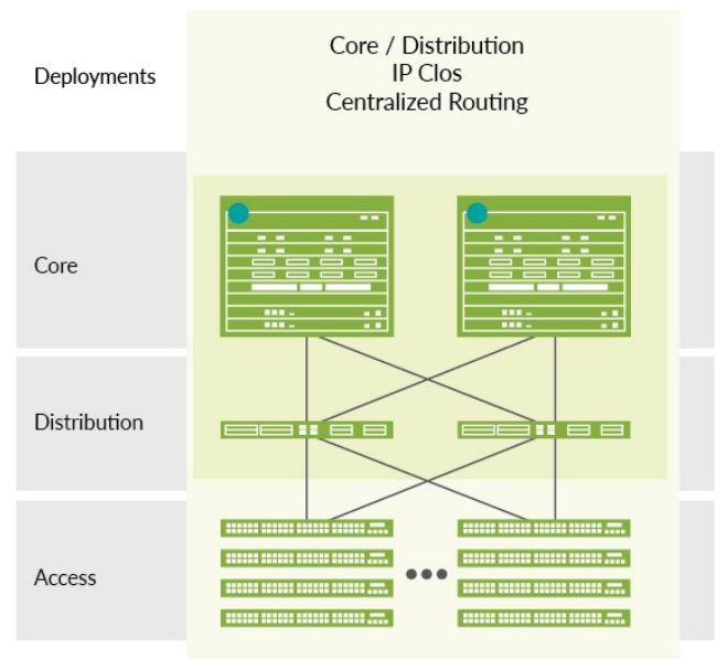
Figure 4: The EX4600 provides 10GbE server access in the data center.
